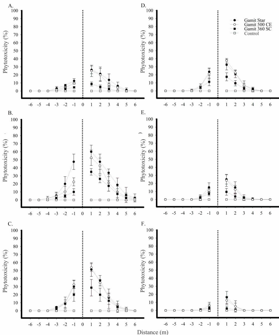
Figure 2. Phytotoxicity in sorghum plants during the 2011/2012 growing season at 2 (A), 5 (B) and 10 (C) 14 (D), 20 (E) and 24 (F) days after application at distances (m) from the point of application (0), of three clomazone formulations: Gamit 360 CS ® , Gamit 500 EC ® and Gamit Star ® . Positive values represent the direction of the prevailing wind and the negative values the opposite direction. The dots represent the mean values of the replications, and the bars the respective mean confidence intervals at 95% probability level.
