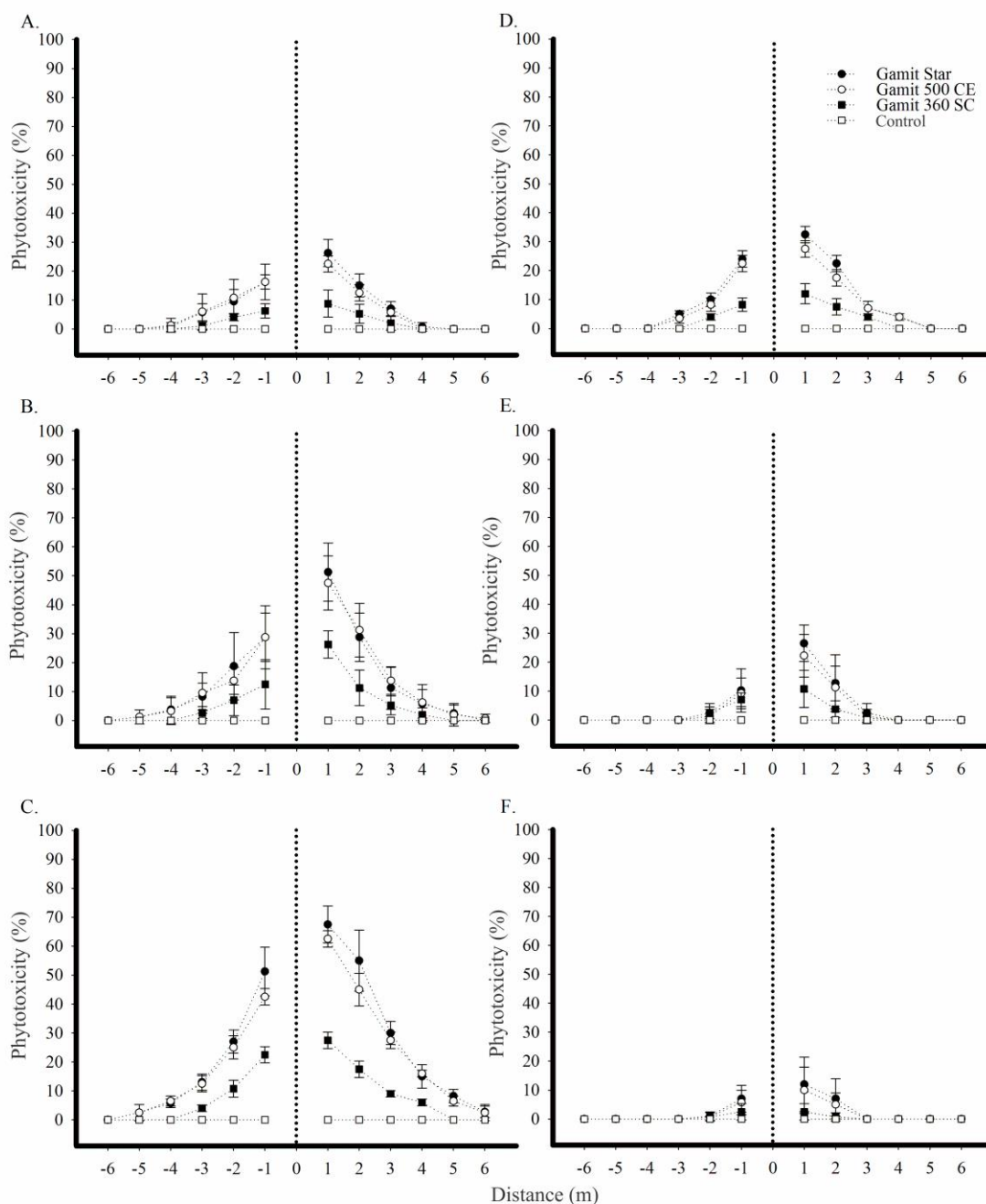
Figure 3. Phytotoxicity in sorghum plants during the 2012/2013 growing season at 2 (A), 5 (B) and 10 (C), 14 (D), 20 (E) and 24 (F) days after application at the respective distances (m) from the application (0) of three clomazone formulations: Gamit 360 CS ® , Gamit 500 EC ® and Gamit Star ® . Positive values represent the direction of the prevailing wind, and the negative values the opposite direction. The dots represent the mean values of the replications, and the bars the respective mean confidence intervals at 95% probability.
