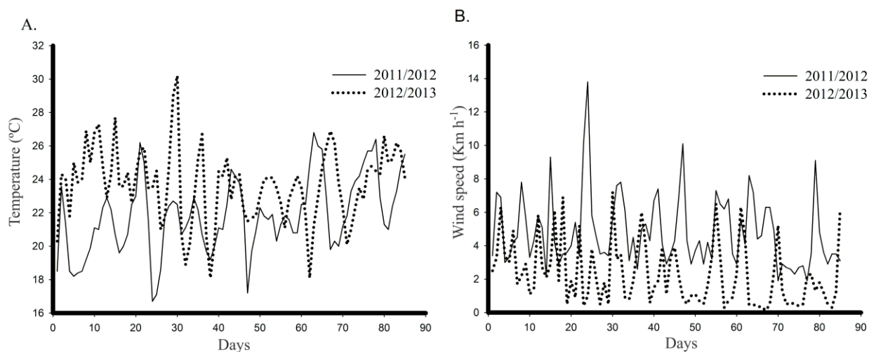
Figure 4. Daily mean air temperature (°C) (A) and daily mean wind speed (km h -1 ) (B) during the experimental periods (2011/2012 and 2012/2013 growing seasons), after sowing sorghum, collected by thermo-hygro-anemometers.
