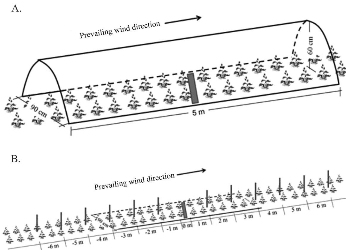
Figure 1. Schematic plot arrangement, showing the tray allocation containing soil treated with herbicide (represented by the gray rectangle) (A) and stakes placed one meter apart from each other, from the herbicide application point (B).
